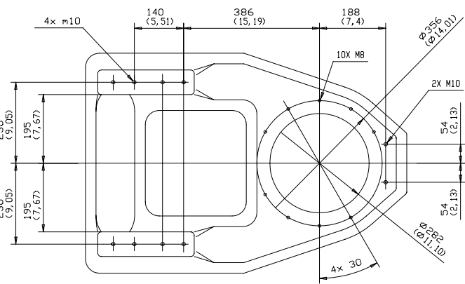
ENGINE BED
